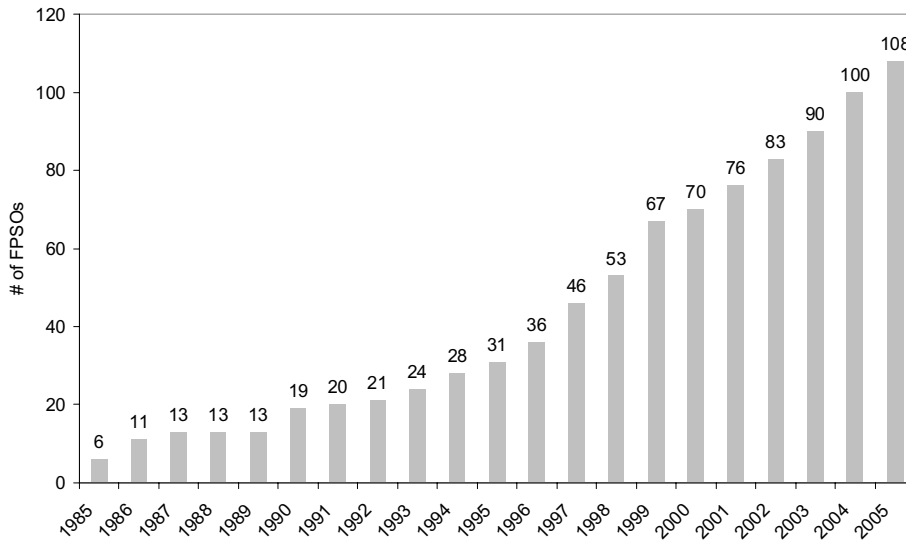
Figure 10-8: 20 year development of the worldwide FPSO fleet (no. of units by year end)
